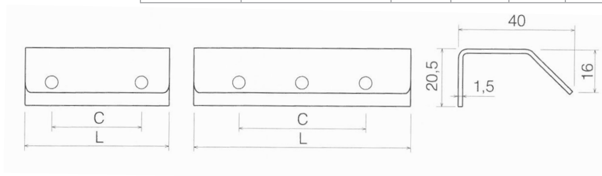
Winkelgriff IN-380
